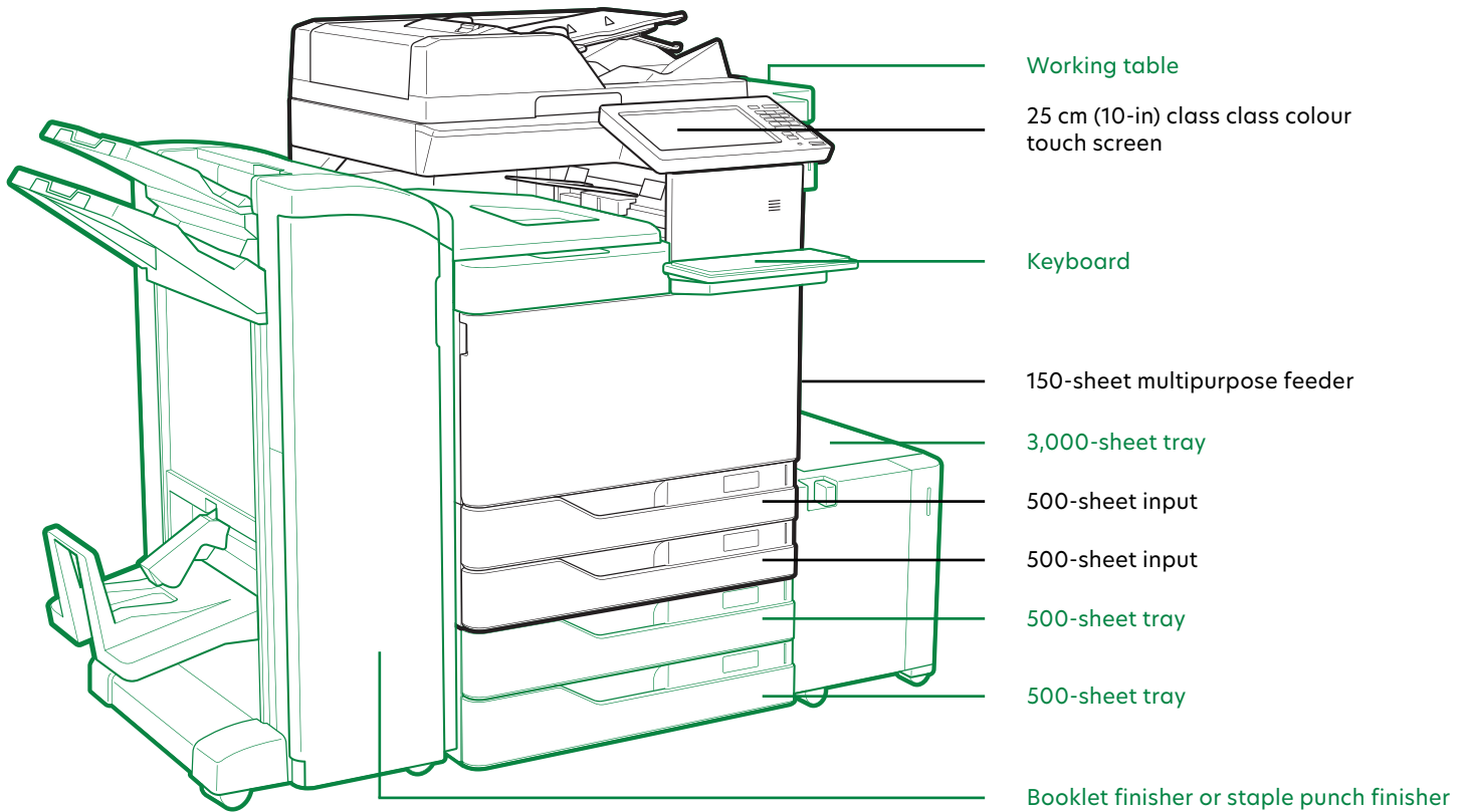
Staple finisher - not compatible with XC9265
